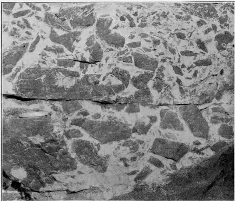
Brecciated quartzite near Ablemans in the Upper Narrows. The darker parts are quartzite, the lighter parts the cementing quartz.
