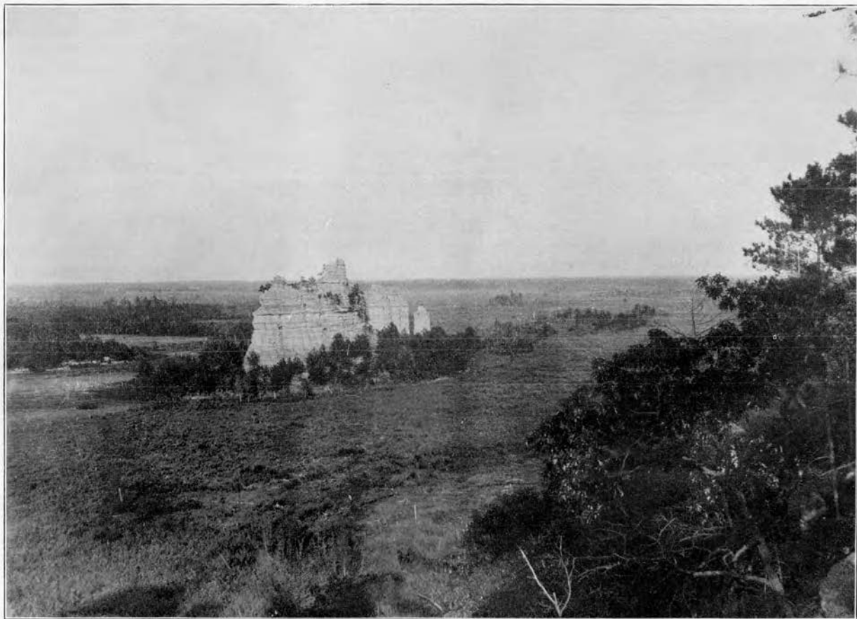
Castle Rock near Camp Douglas. In this view the relation of the erosion remnant to the extensive base-leveled surface is well shown.
