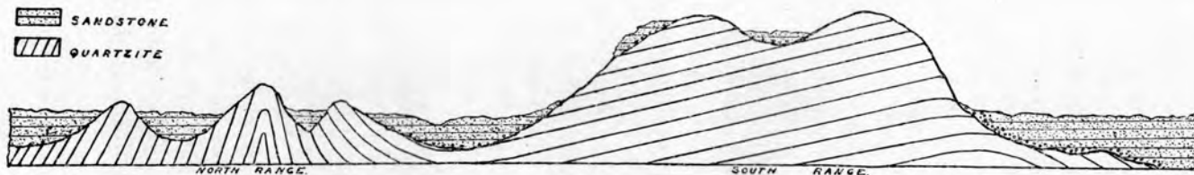
FIG. 5.—A diagrammatic section showing the relation of the sandstone to the quartzite.
