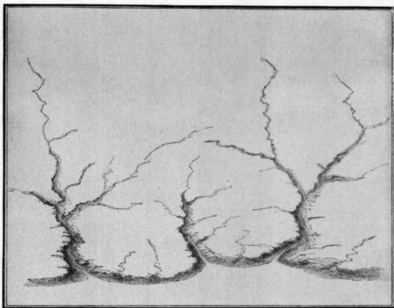
FIG. 3. Young valleys.
