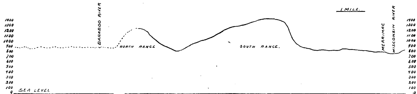
FIG. 2.—Profile north from Merrimac across the quartzite ranges. The dotted continuation northward represents the extension of the profile beyond the topographic map, Plate XXXVII.
