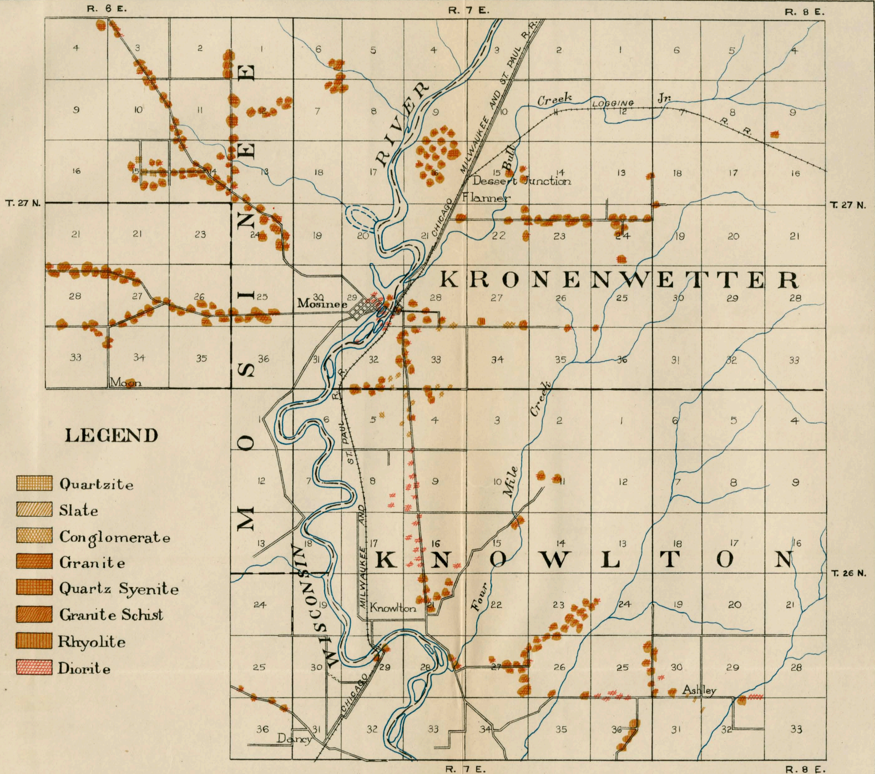
MAP SHOWING ROCK OUTCROPS IN VICINITY OF MOSINEE
