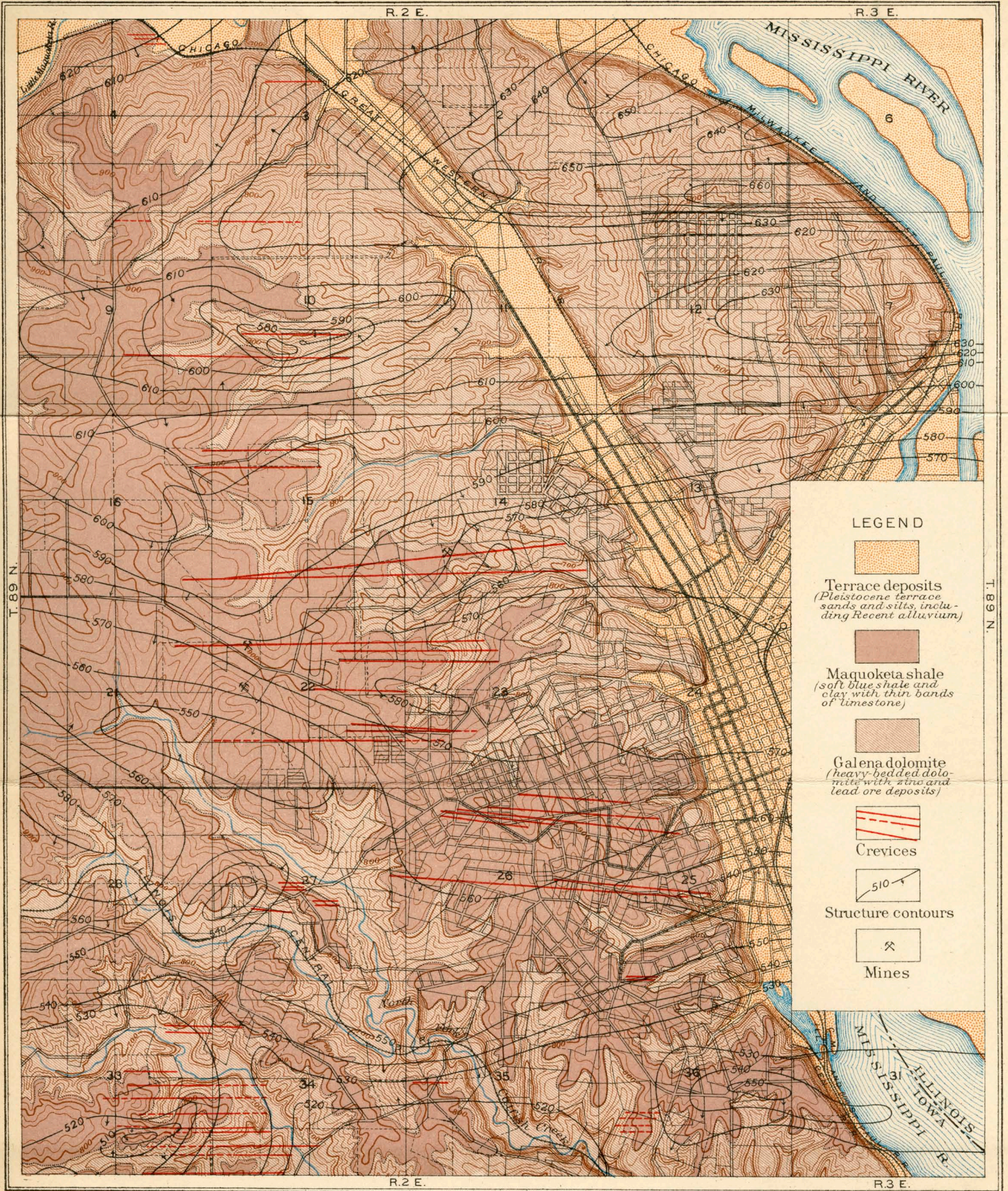
MAP SHOWING GEOLOGY AND TOPOGRAPHY OF THE DUBUQUE AREA, BY E. E. ELLIS with structural contours on the base of the Galena dolomite by H. F. Bain and principal crevices by W. H. Guilford
