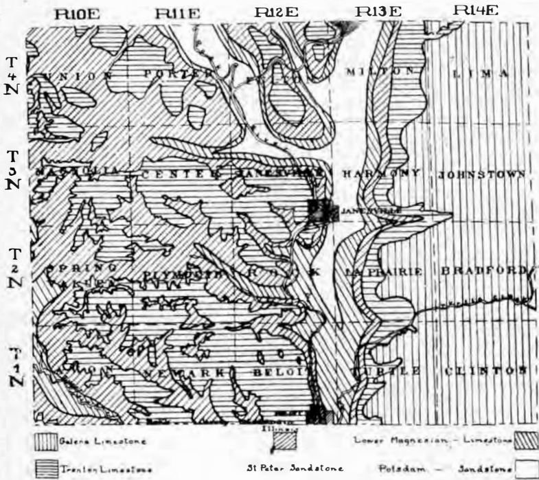
Fig. 3.—Sketch showing surface rock formations in Rock County.
