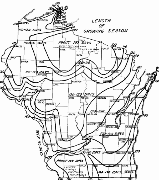
FIG. 2. Map showing length of growing season.
