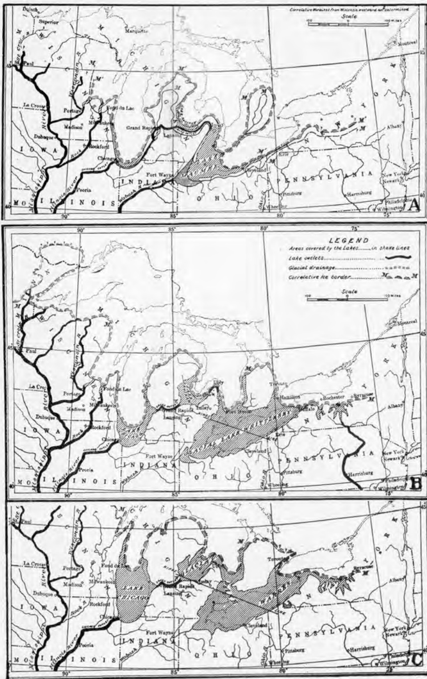
Fig. 6—Position of the glacial lakes at various stages in the development of the Great Lakes. Different outlets were used at different stages. Note the increase in the size of the lakes as the ice-front retreated northward. (Taylor and Leverett.)
