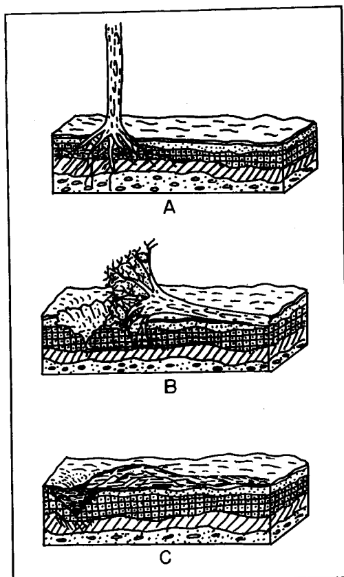
Figure 19. Stages in evolution of a "cradle-knoll".
