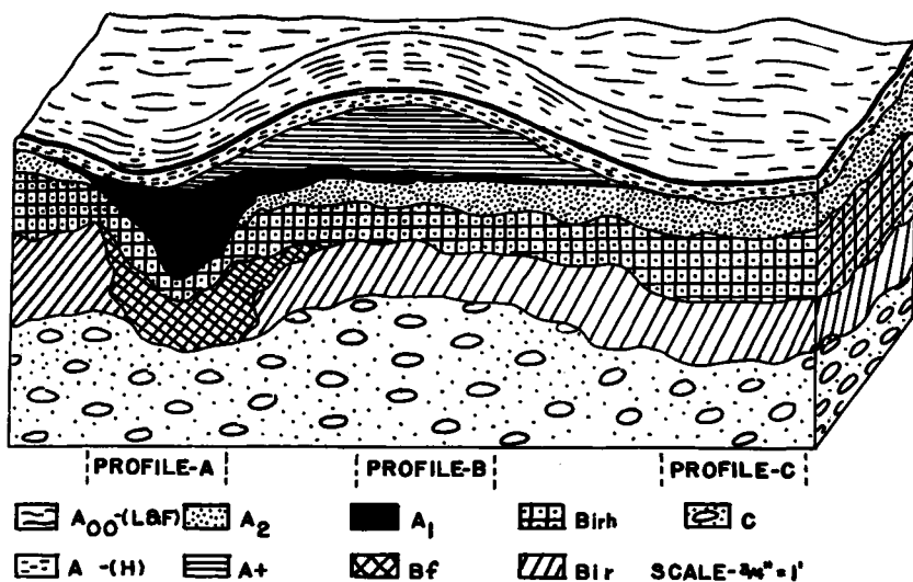
Figure 20. Cross-section of a "cradle-knoll".
