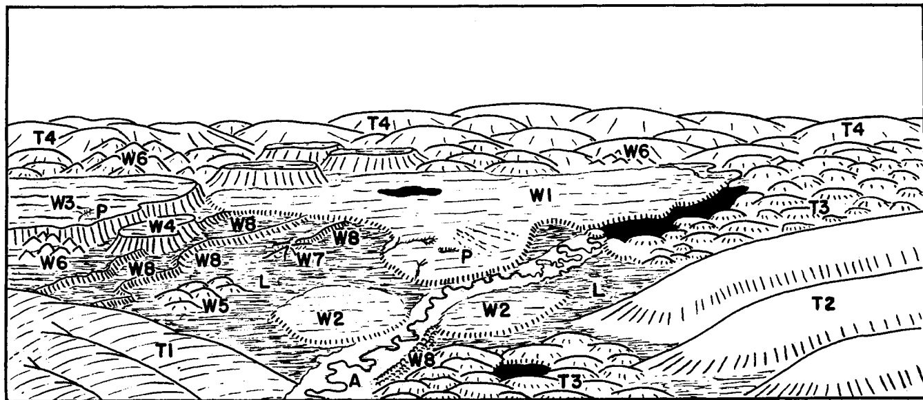
Figure 13. Some land forms of Oneida County, Wisconsin. See page 26 for the legend for symbols.
