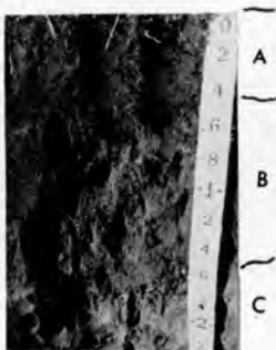
Figure 4. Pence sandy loam on an undulating outwash plain. The sandy loam plow layer (A p ) is underlain by a sandy loam horizon (B) which has been
