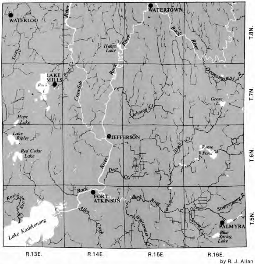
Figure 18. Lakes and streams.
