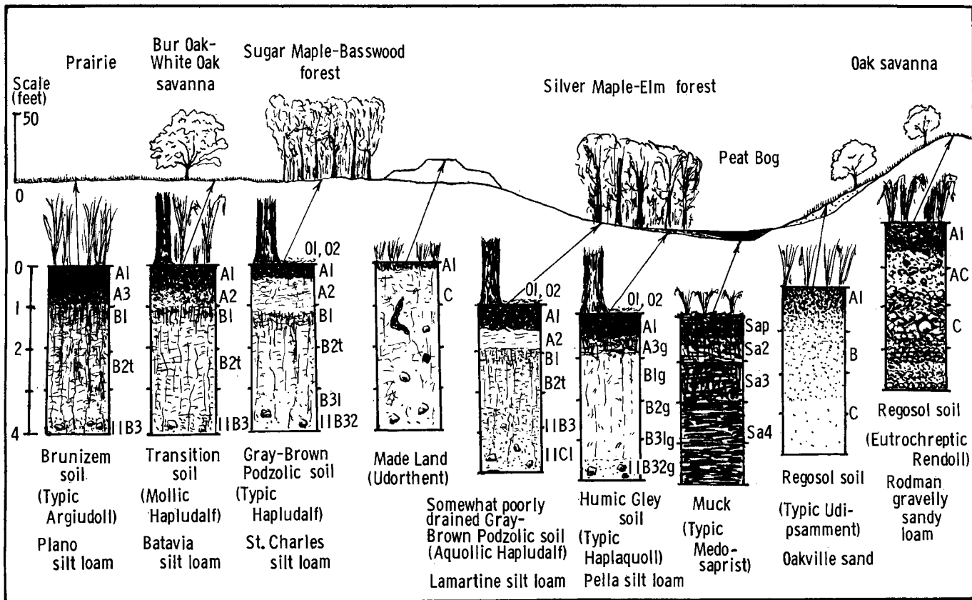
Figure 7. Nine representative soil profiles of Jefferson County, Wisconsin, with landscape positions indicated (terms in parentheses are from the new USDA Comprehensive Soil Classification).
