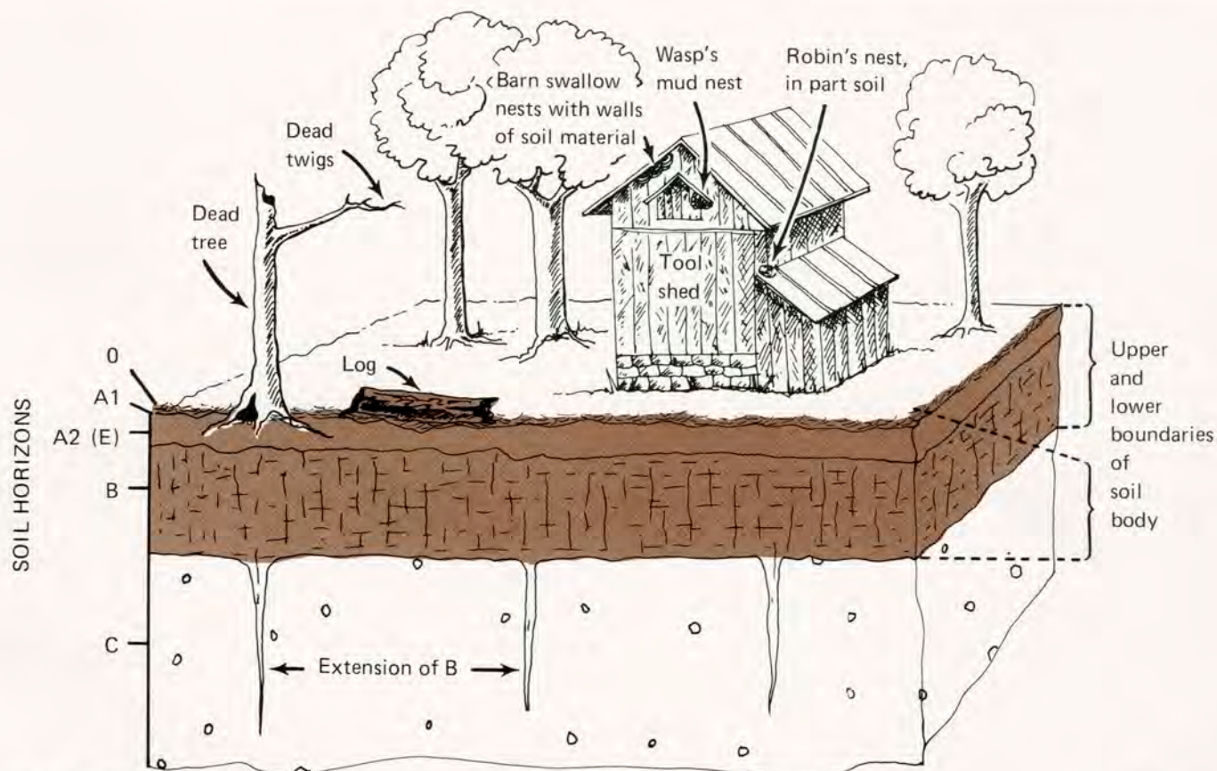
Figure 4. Block diagram showing the upper and lower boundaries of a true soil body as distinct from geologic substratum (C horizon) and vegetation and structures that are above-ground.
