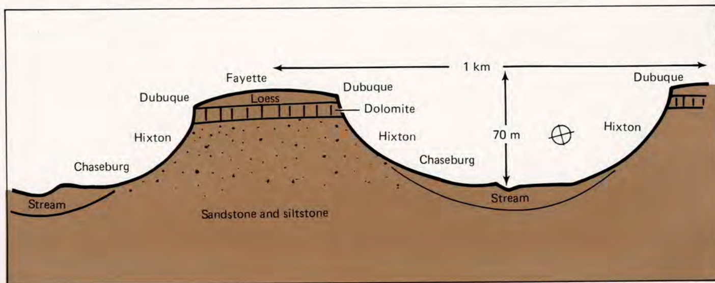
Figure 13. Arrangement of some soils on an idealized landscape of western Wisconsin.
