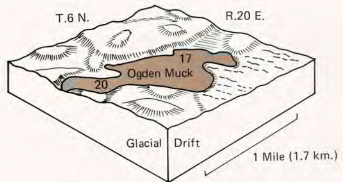
Figure 3. Block diagram of a portion of a soil landscape in Waukesha County, Wisconsin showing a body of Ogden muck, in sections 17 and 20, Township 6 North, Range 20 East.
