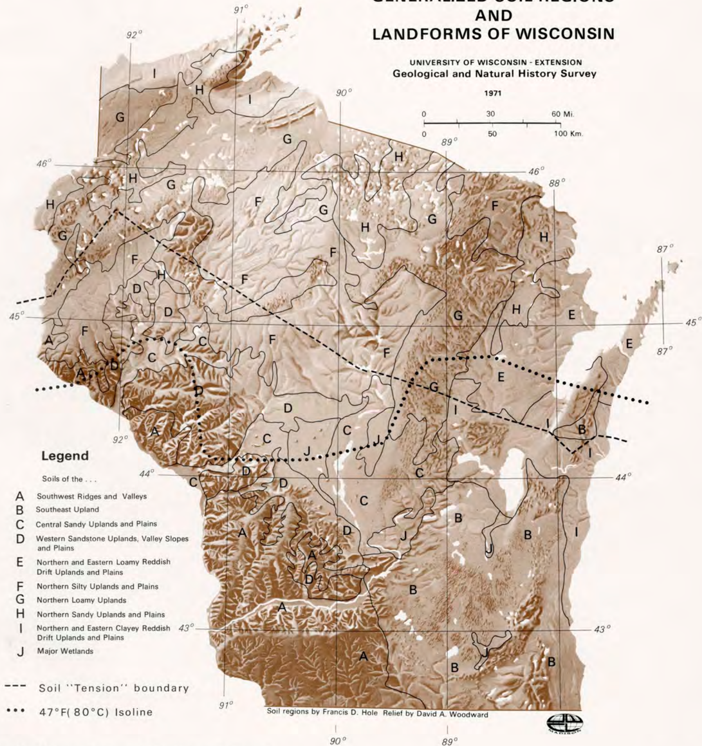
Figure 17. Major soil regions and landforms of Wisconsin.
