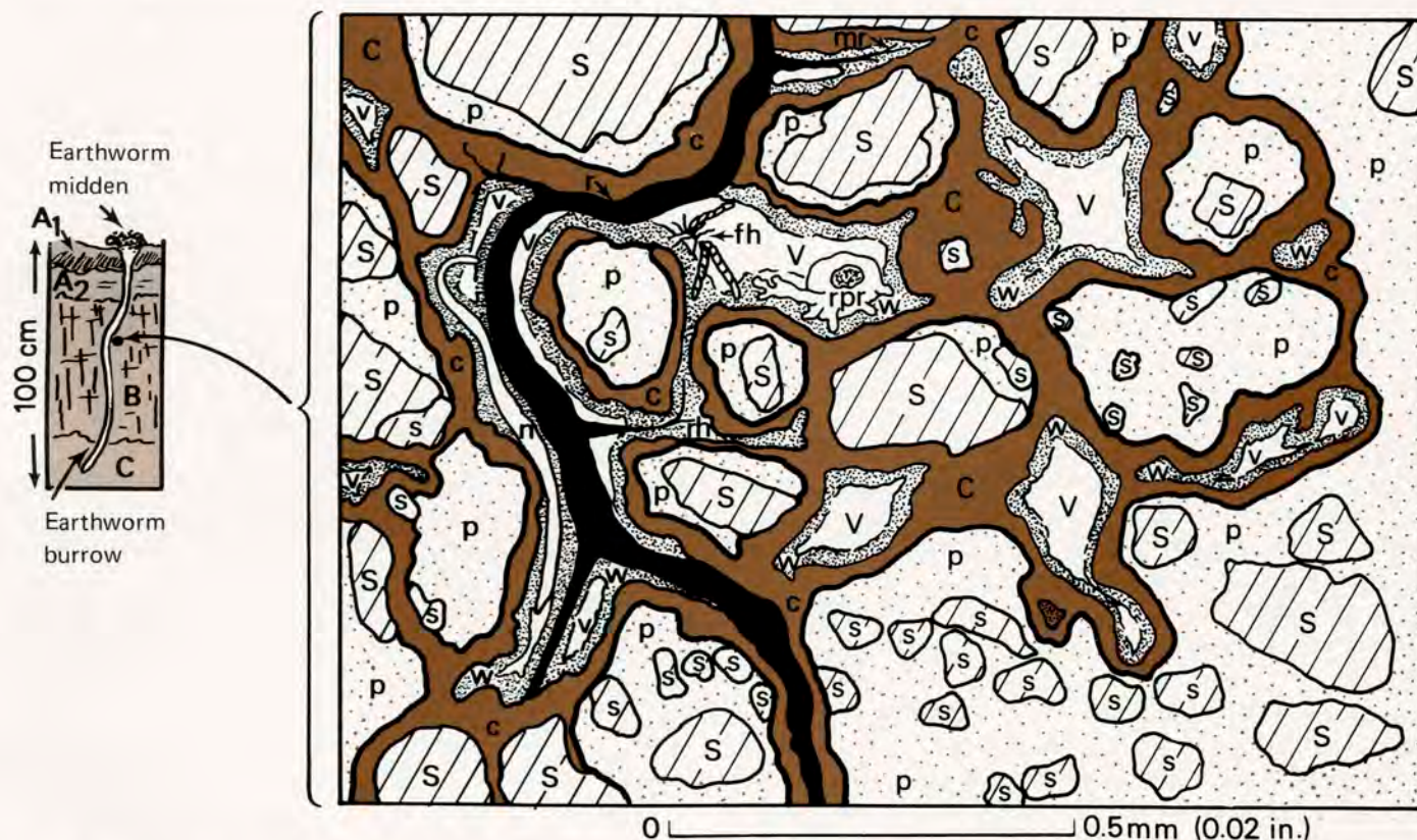
Figure 1. Diagrammatic cross-section of (left) a soil pedon with A1, A2, B and C horizons, earthworm burrow and midden; and (right) 1.5 mm 2 of fresh, undisturbed subsoil (B horizon). Legend: c = clay skins (argillans) coating walls of voids; fh = fungal hyphae; mr = mycorrhizum; n = nematode; p = plasma (clay and fine silt) of soil; rpr = amoeba (rhizopodal protozoan), r = live root; rh = root hair; v = air-filled void; w = water film in void; s = skeletal sand grains.
