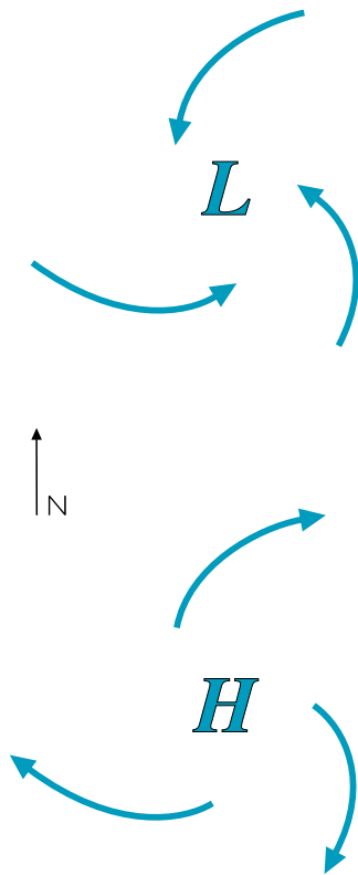
Figure 1. Wind patterns around low- and high-pressure centers.
