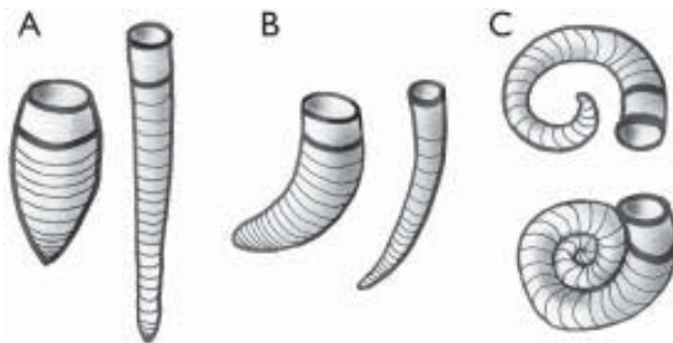
Figure 15. Morphologies of fossil cephalopods. A: Straight. B: Crescent-shaped. C: Coiled.
