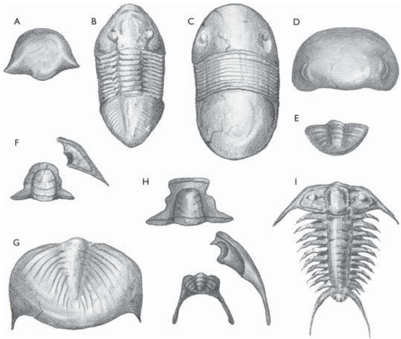
Plate 7. Trilobite fossils. A: Cephalon of Illaeus , a common trilobite in Ordovician rock. The cephalon is similar in shape to a strophomenid brachiopod [2.5 cm]. B: Complete specimen of the Ordovician trilobite Isotelus . It has a more triangular cephalon and pygidium than Bumastus , and a more pronounced axial lobe [5 cm]. C: Bumastus , a Ordovician mud-burrowing trilobite with a broad, rounded cephalon and pygidium [6.5 cm]. D: Large cephalon of Bumastus [4 cm]. E and F: Stubby, rounded pygidium and disarticulated cephalon of the Cambrian trilobite Conaspis . The glabella is more rounded than that of Crepicephalus (shown on this plate as H) [3 cm]. G: Large, egg-shaped pygidium of the upper Cambrian trilobite Dikelocephalus [6 cm]. The pygidium looks similar to a fish tail. H: Molted parts of the Cambrian trilobite Crepicephalus . The glabella is more squared than that of Conaspis . Extensions of the pygidium make it look similar to a swallowtail butterfly wing [3 cm]. I: The Ordovician trilobite Ceraurus , showing the characteristic tail spines and pronounced “ribs” of the pleural lobes [4 cm].
