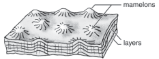
Figure 19. Stromatoporoid anatomy.
