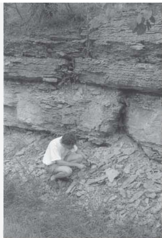
Figure 4. A paleontologist collecting Middle Ordovician fossils from a roadcut in southwestern Wisconsin.
