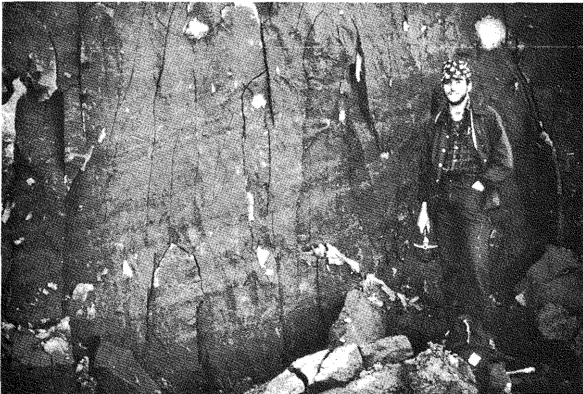
Figure 10.--Clay stringers in the Hanson Creek Member. Ice flowed from left to right. Exposure is 1.5 km west of the mouth of the Amnicon River. Figure reproduced with the permission of The Journal of Sedimentary Petrology, v. 53, p. 859-874, fig. 4.
