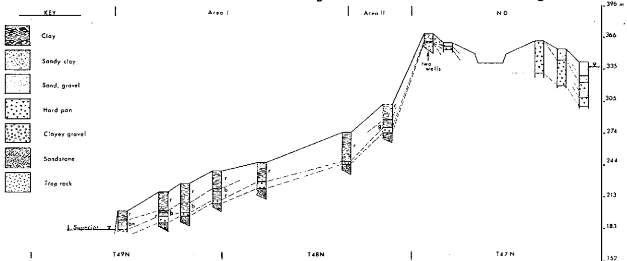
Figure 16.--Subsurface cross section--Haukkala Creek to Lake Nebagamon. Areas I and II shown at the top of the figure are the type areas defined by Mengel and Brown (1979); ND--not defined. The Douglas Member is correlated with the surface and near-surface unit containing red clay (r); the Hanson Creek Member is correlated with units containing gray clay (g), brown clay (bn), and red clay (r) underlying blue clay (b); the Jardine Creek Member is correlated with units containing hard pan and clayey gravel. Note the southern limit of the Hanson Creek Member at the southern edge of T. 48 N. and the two wells at about 366 m encountering red clay. (The highest proglacial lake level was 341 m.) Also note the buried valley south of these wells in T. 47 N.
