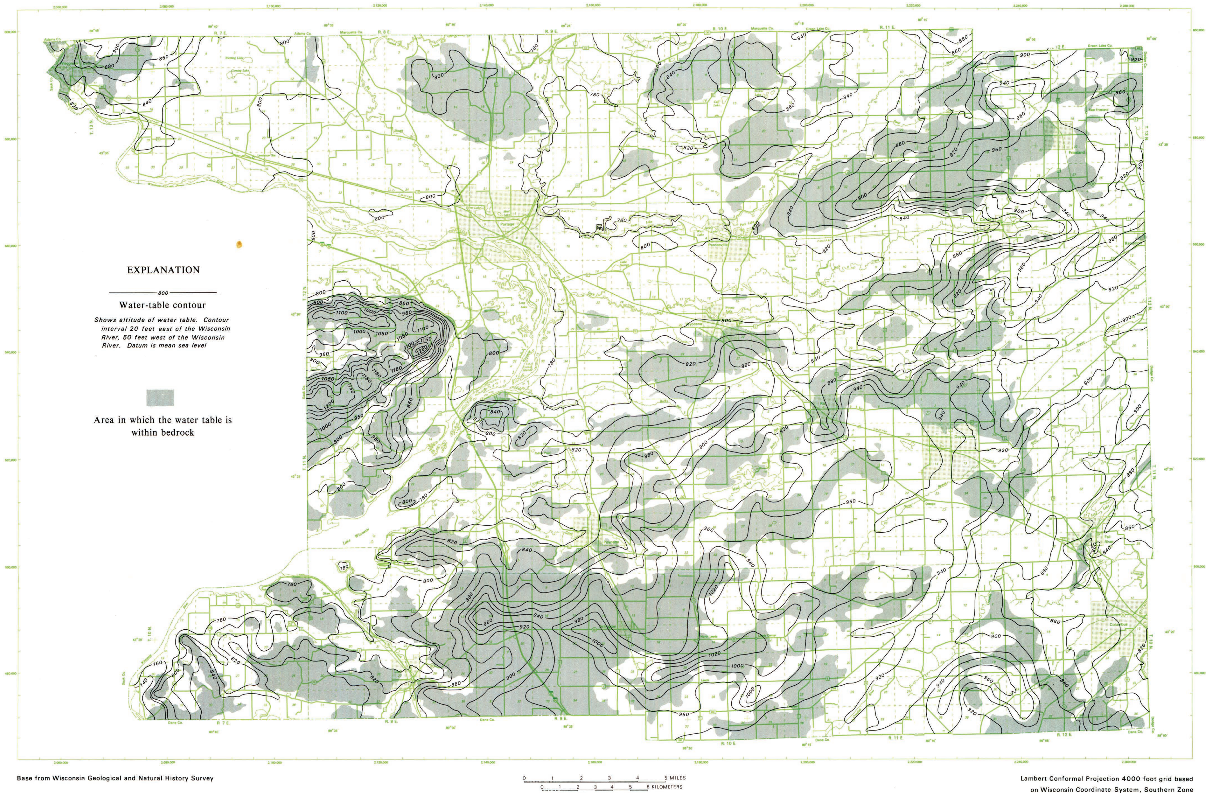
Plate 1. Water-table map of Columbia County, Wisconsin, 1974.
