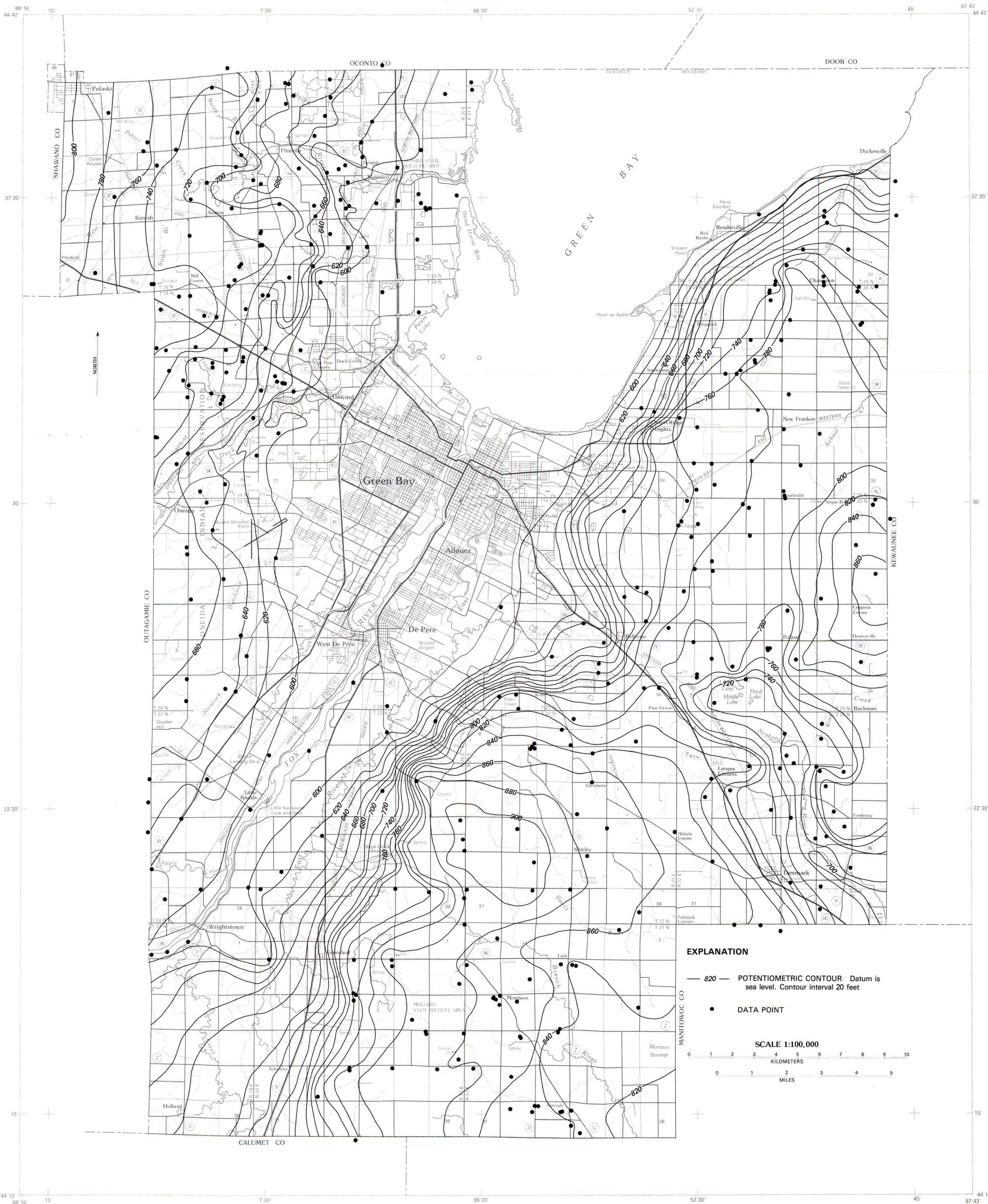
PLATE 1. POTENTIOMETRIC SURFACE OF UPPER AQUIFER, BROWN COUNTY, WISCONSIN, 1980
