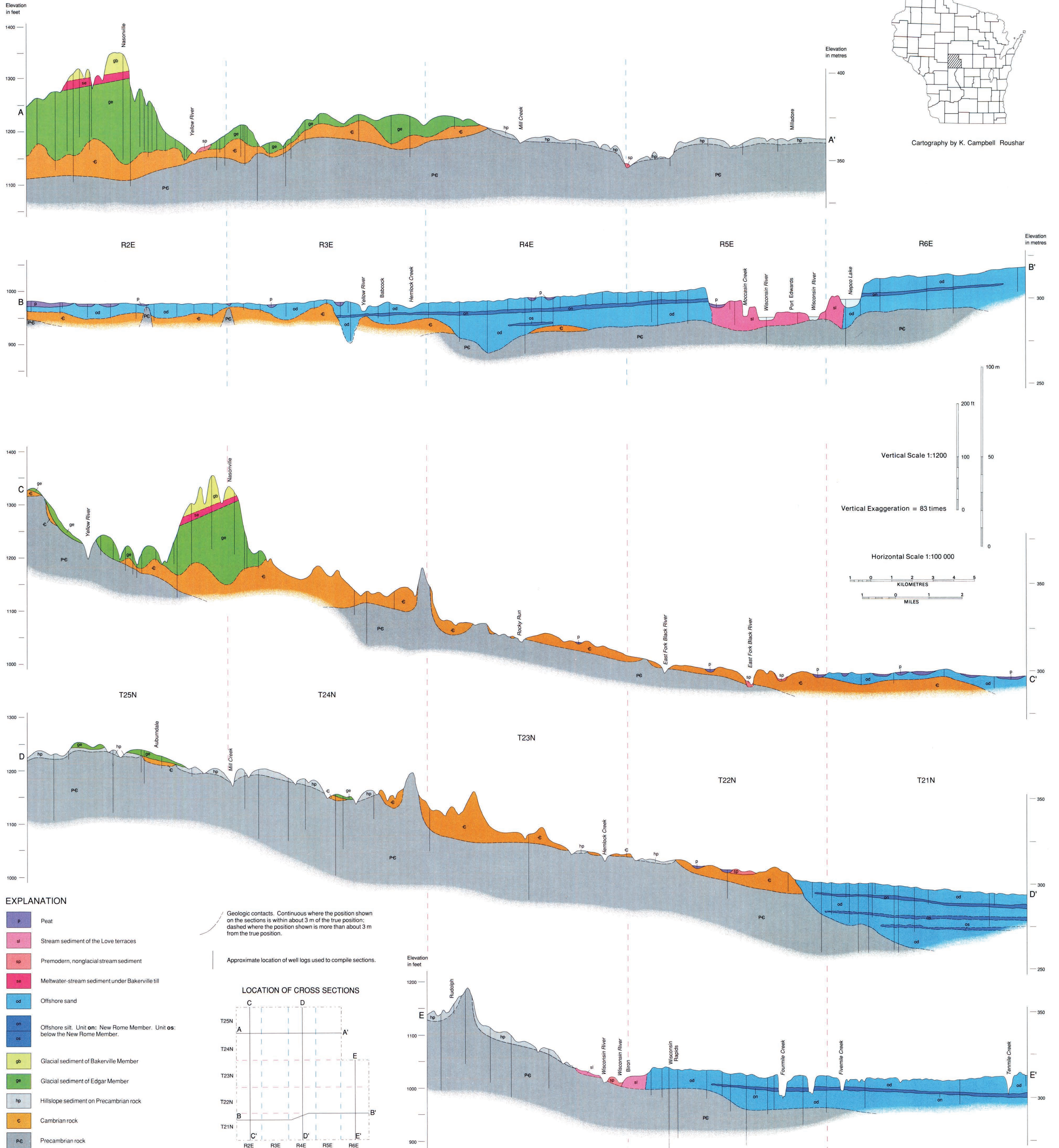
PLATE 2. GEOLOGIC CROSS SECTIONS OF WOOD COUNTY, WISCONSIN
