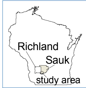
Figure 1. Study area in Sauk and Richland Counties (above) and topography (left). Blue shaded area indicates extent of flooding in 2008. White border is the extent of the MODFLOW model domain.
